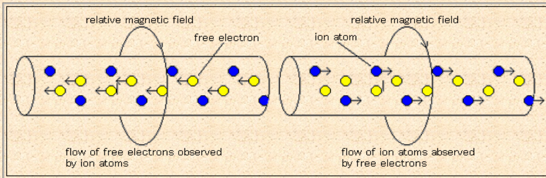
(CHART 1) conduction current
