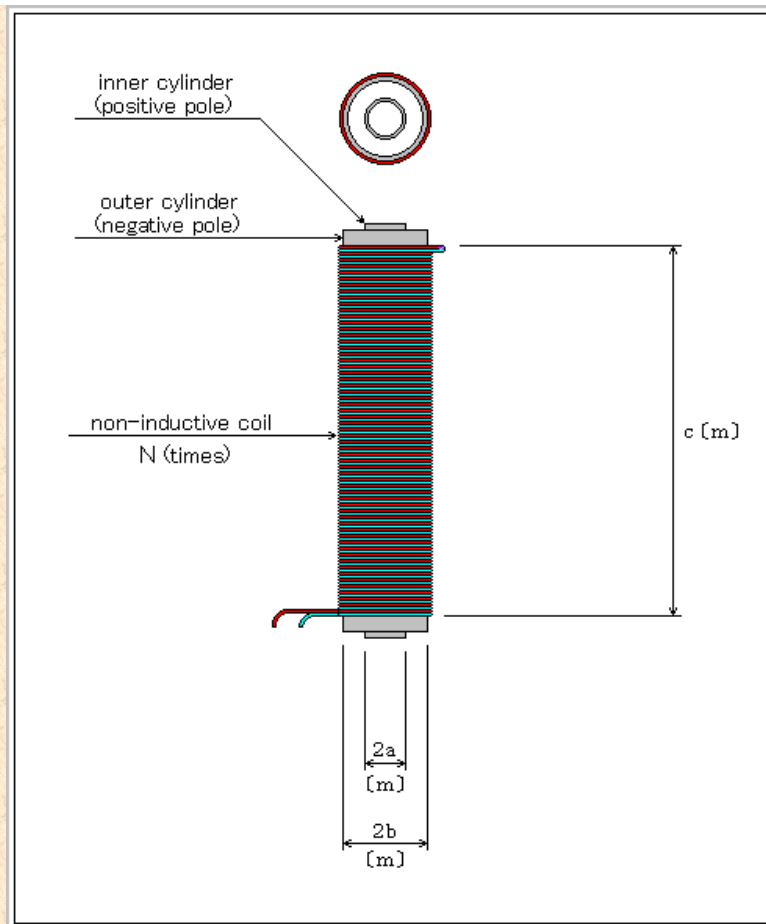
(CHART 6) NEGATIVE INDUCTOR
